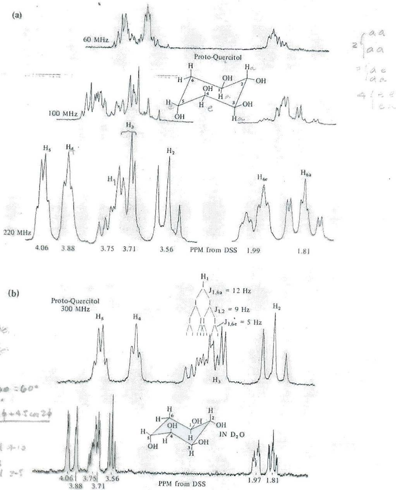
Fig. 4.19 (a) 60-, 100-, and 220-MHz spectra of proto -quercitol in D 2 O. (b) 300-MHz spectrum of proto -quercitol in D 2 O. [Reproduced from Ref. 1, with permission of the American Chemical Society.]
